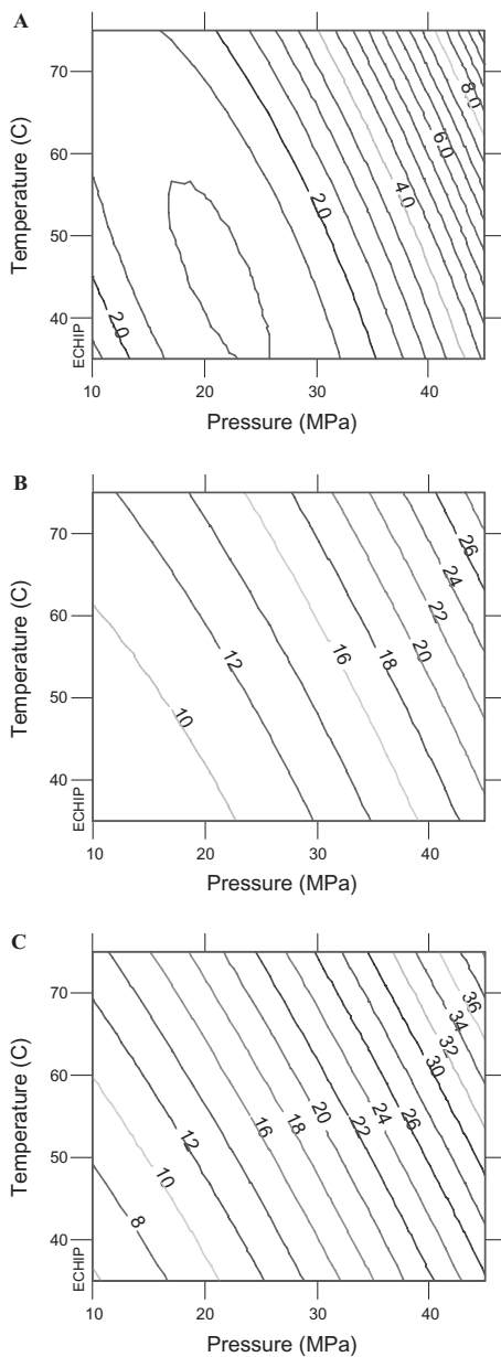
FIG. 1. CONTOUR PLOTS FOR TOTAL FAT CONTENT (%) AS A FUNCTION OF PRESSURE AND TEMPERATURE AT AN EXTRACTION TIME OF (A) 1 h, (B) 6.5 h AND (C) 12 h
