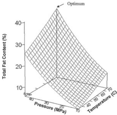
FIG. 2. THREE-DIMENSIONAL CONTOUR PLOT SHOWING THE RESPONSE SURFACE OF TOTAL FAT CONTENT (%) AS A FUNCTION OF PRESSURE AND TEMPERATURE AT AN EXTRACTION TIME OF 12 h
