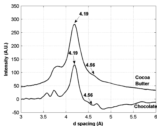
Fig. 4 Comparison between the XRD diffraction pattern of pure cocoa cooled rapidly (50 °C/min), forming \beta crystals, and the XRD diffraction pattern proceeding from the subtraction method applied to milk chocolate cooled under the same conditions
