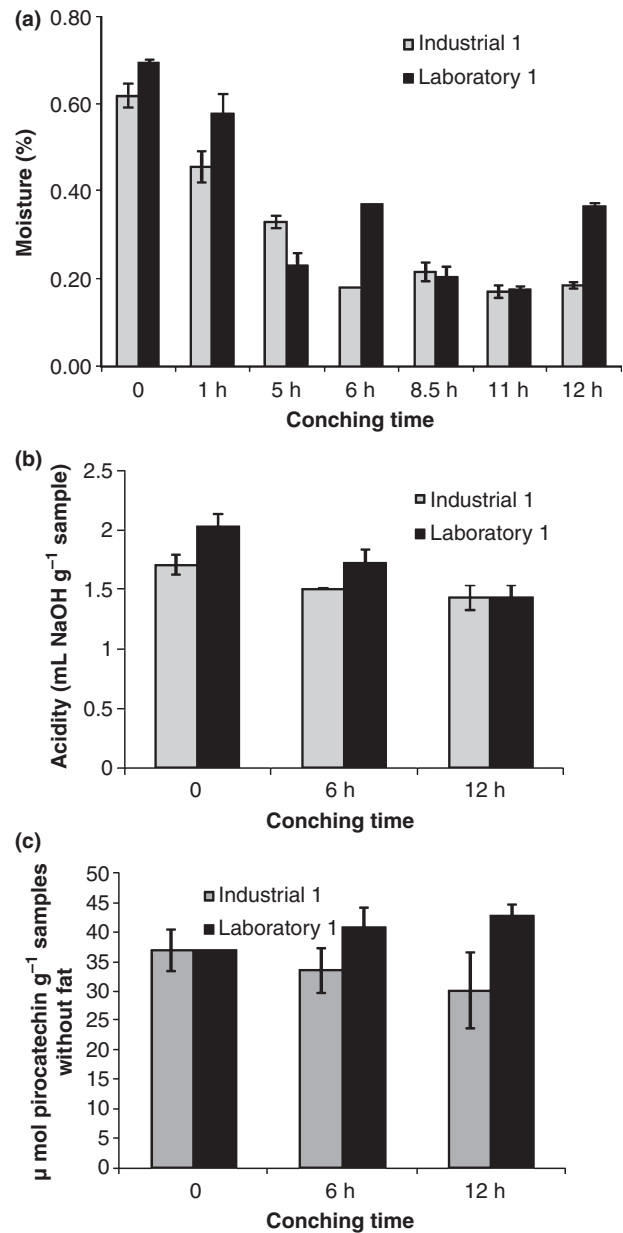
Figure 2 Variation of the moisture (a), acidity (b) and polyphenol concentration (c) in the EXP01, comparing industrial (grey bars) and laboratory (black bars) scale processes. Data are means \pm SEM of duplicate assays.
